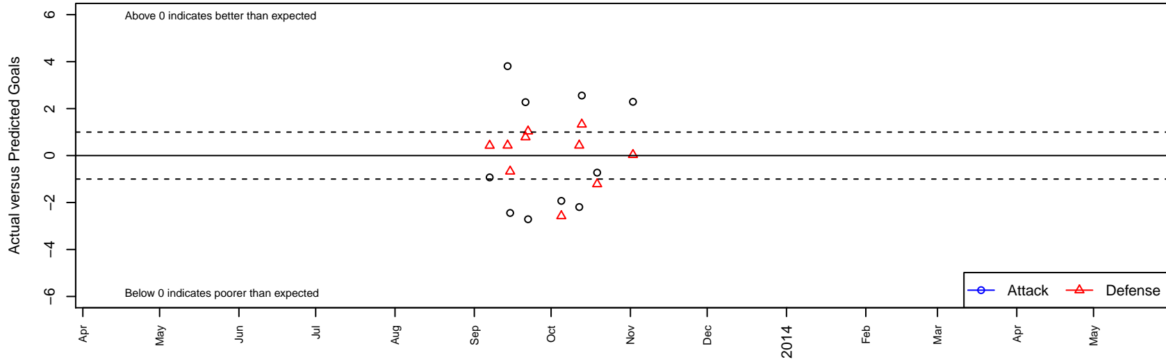
Alum Rock PAC Atlas B98 Dots are actual minus expected GF (blue circles) and GA (red triangles). Blue line is smoothed change in attack strength. Red is smoothed change in defense strength.
